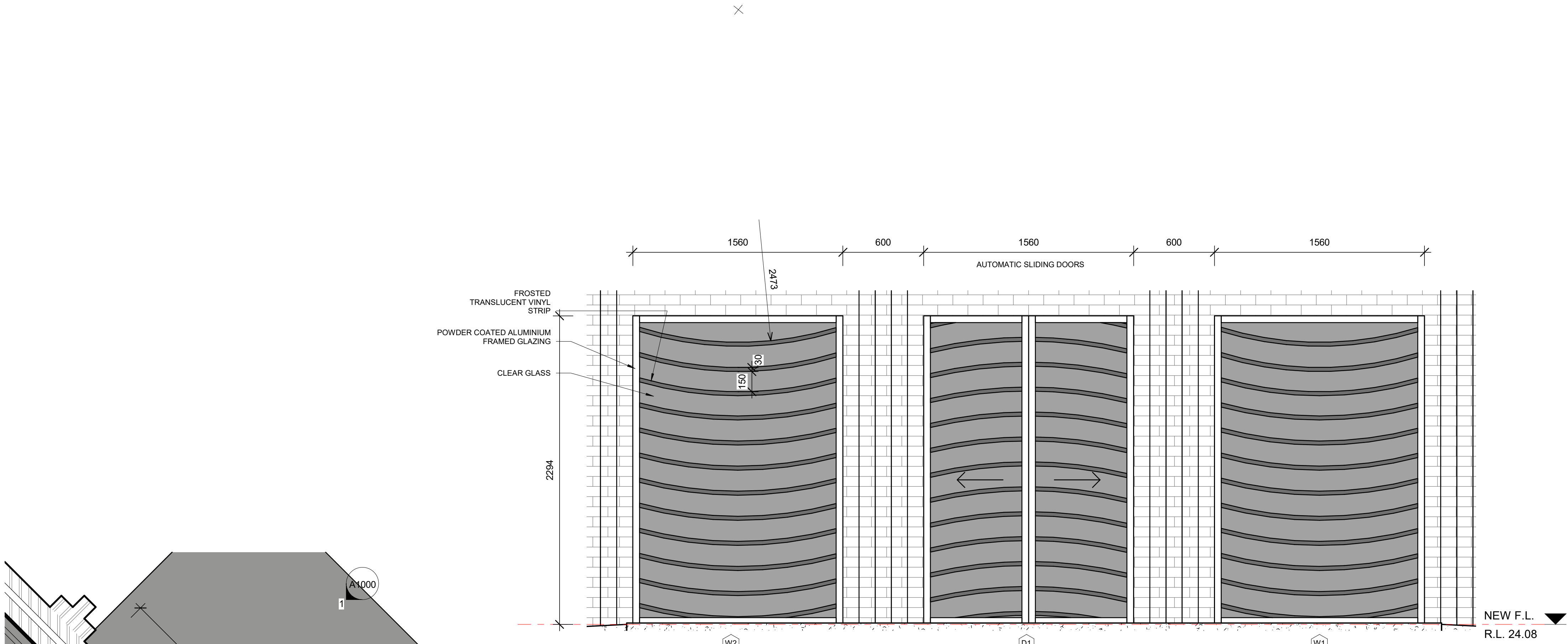
ELEVATION A 1:20
