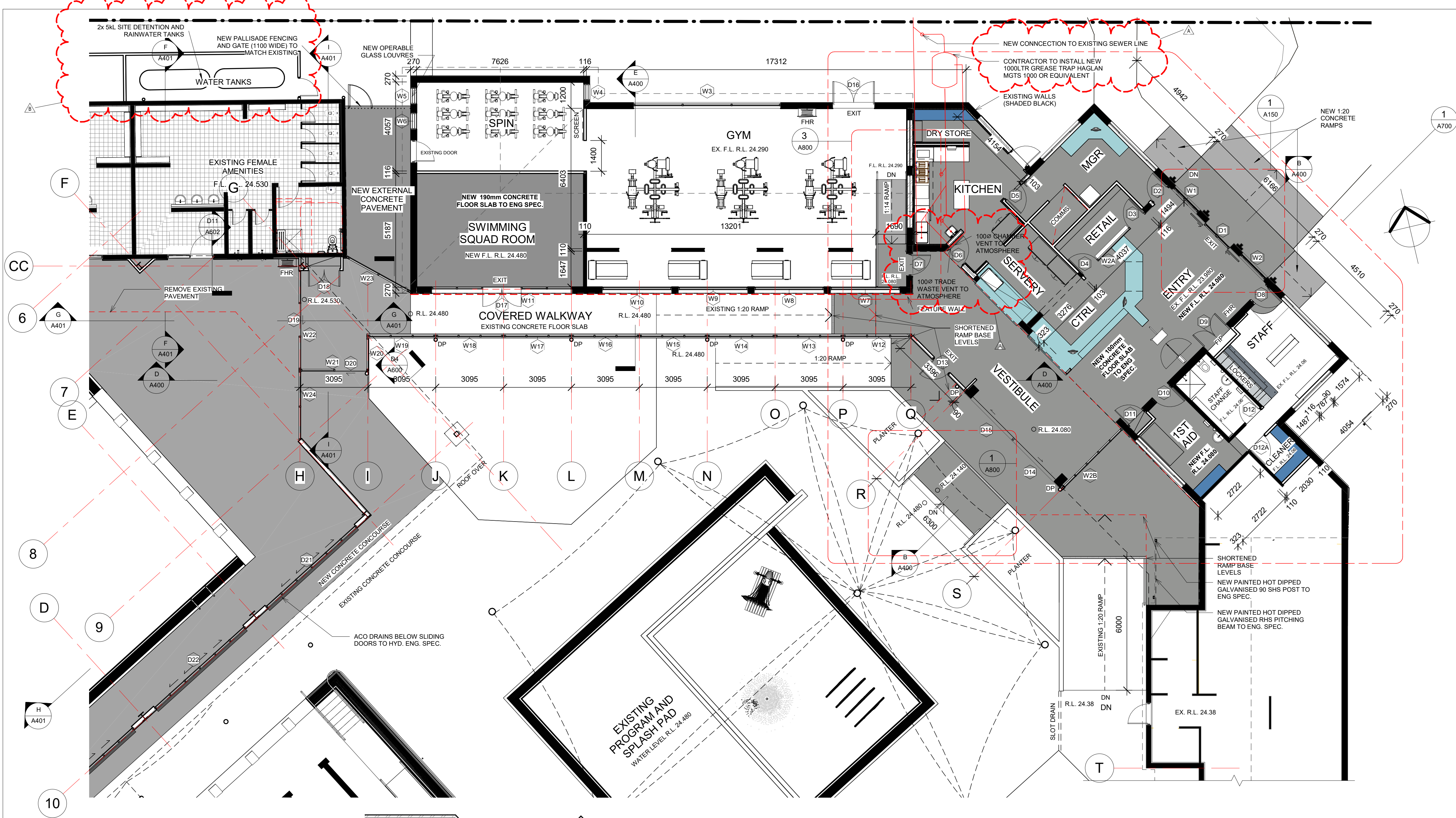
FLOOR PLAN 1 1:100
