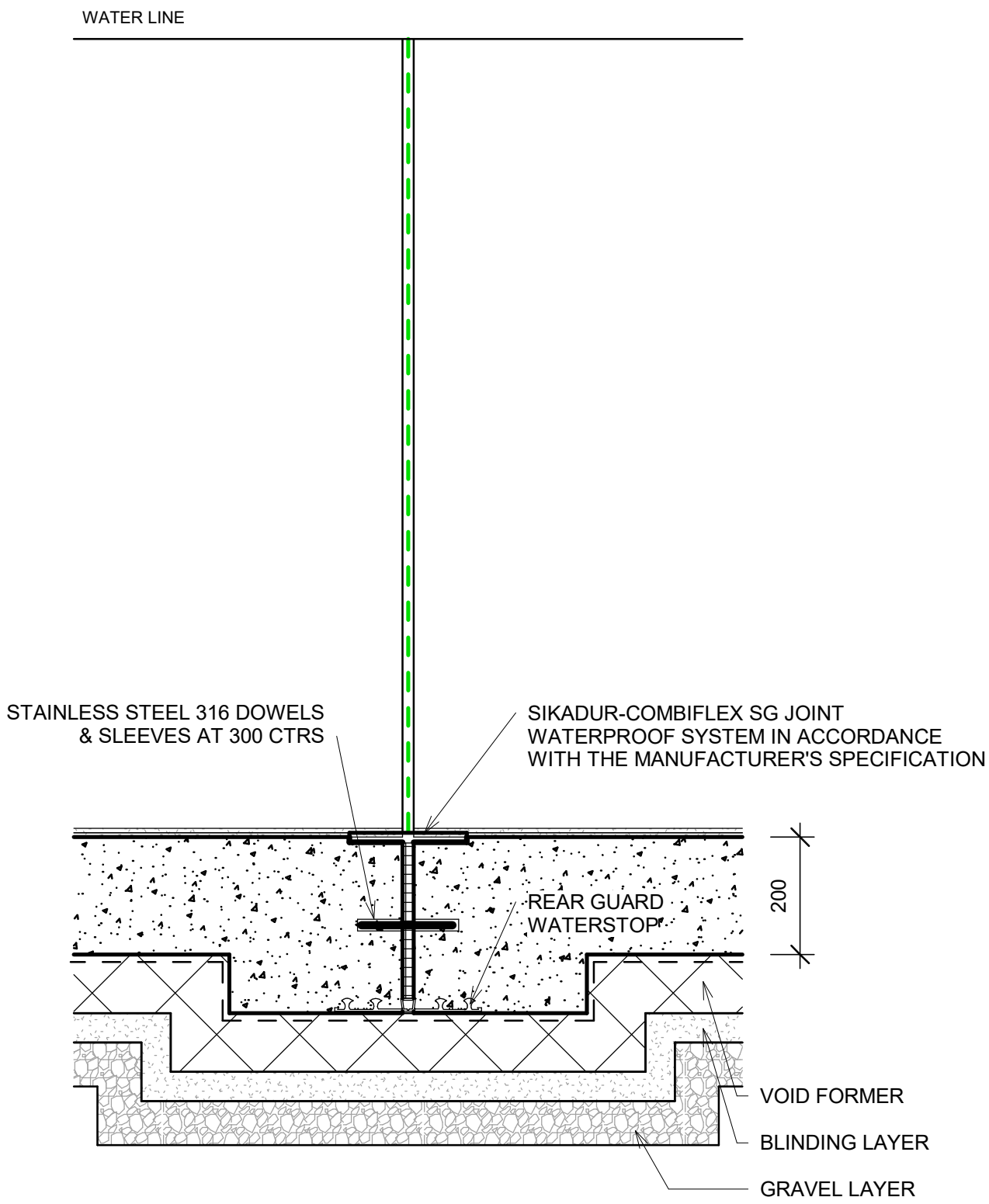
TYPICAL POOL EXPANSION JOINT DETAIL
