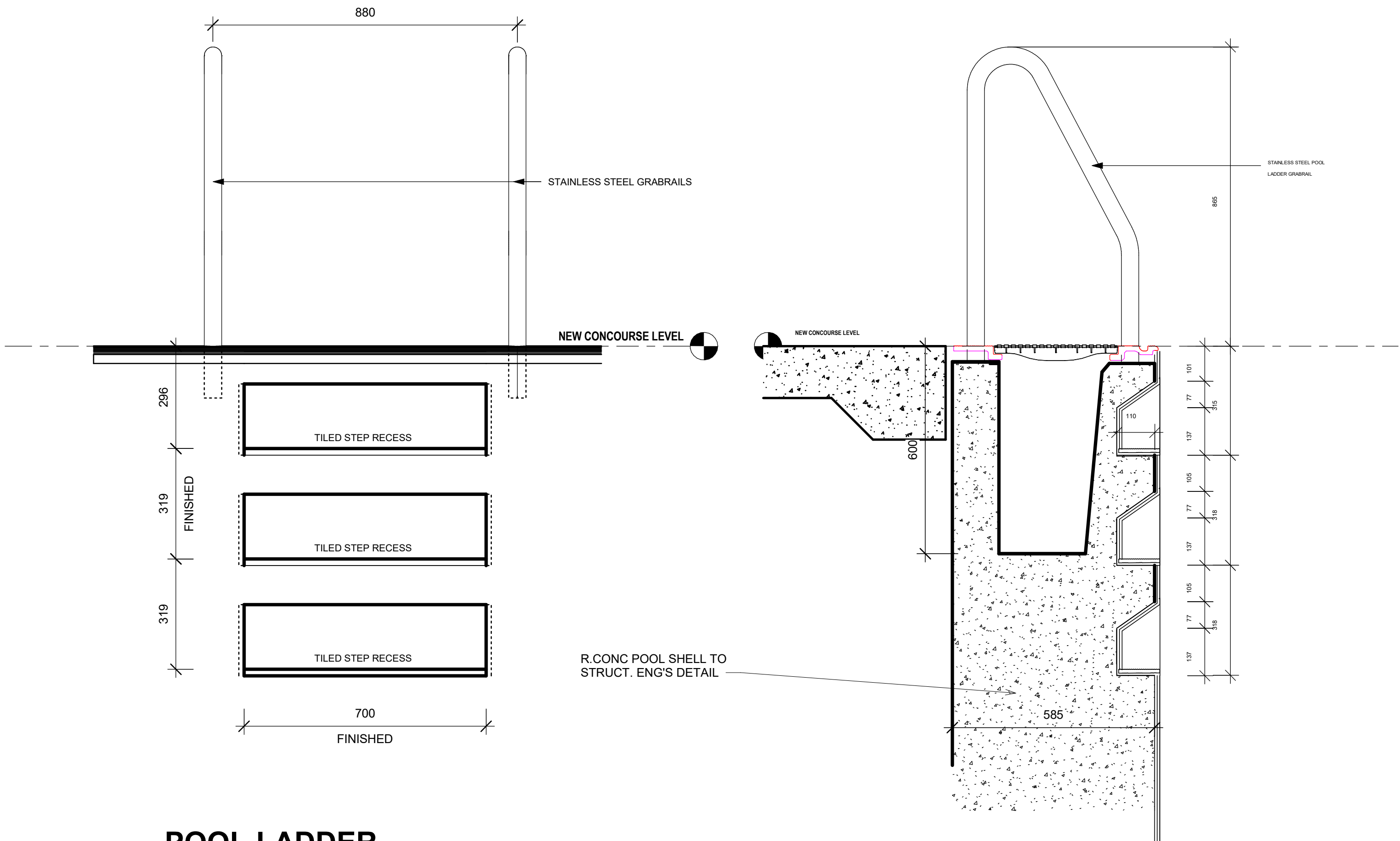
POOL LADDER 1 : 10
